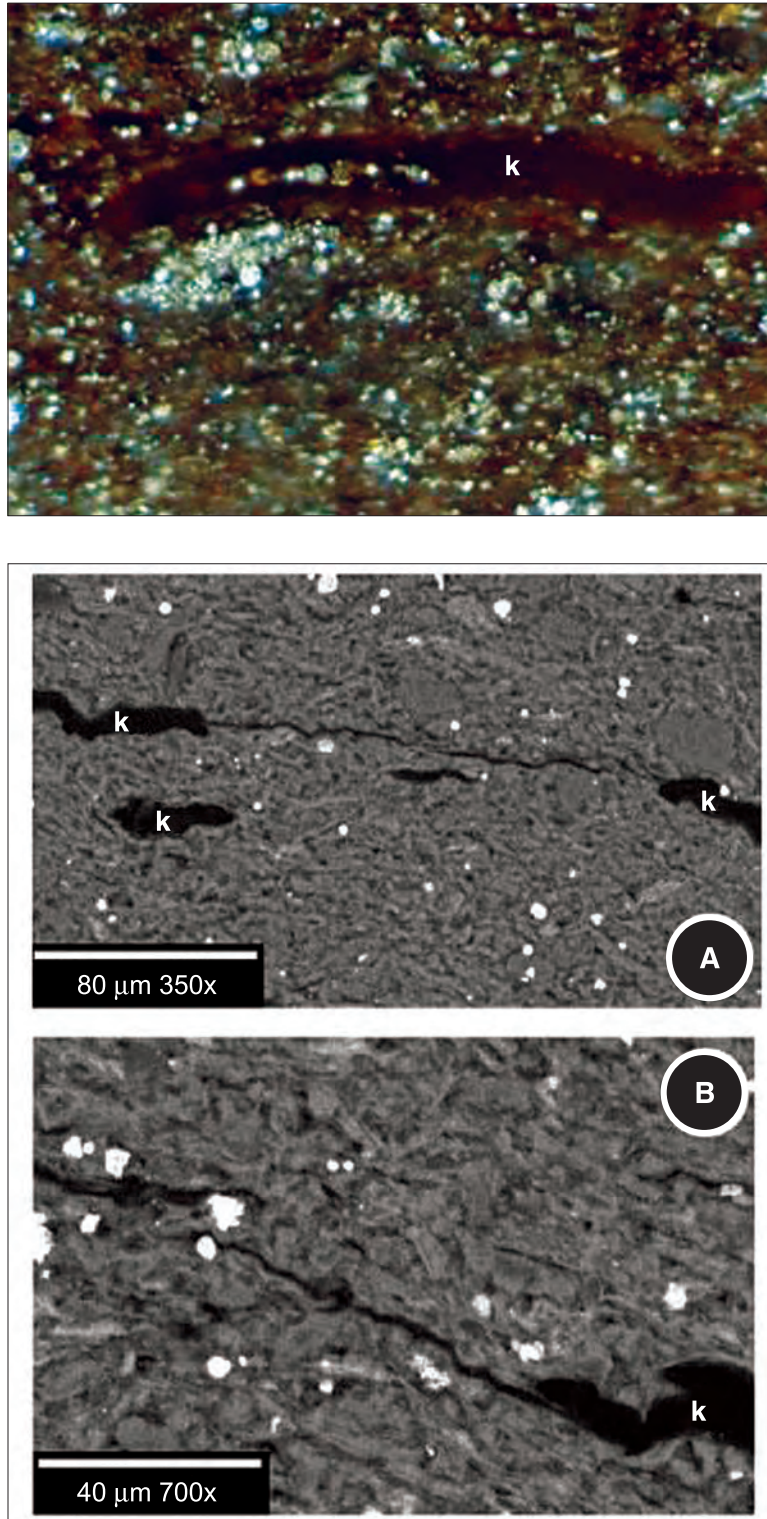
Figure 47. Top: photomicrograph of kerogen particle in Marcellus Shale; modified from Geology.com. Bottom A and B: microfractures propagating between kerogen particles; modified from Engelder and Lash, 2008.
