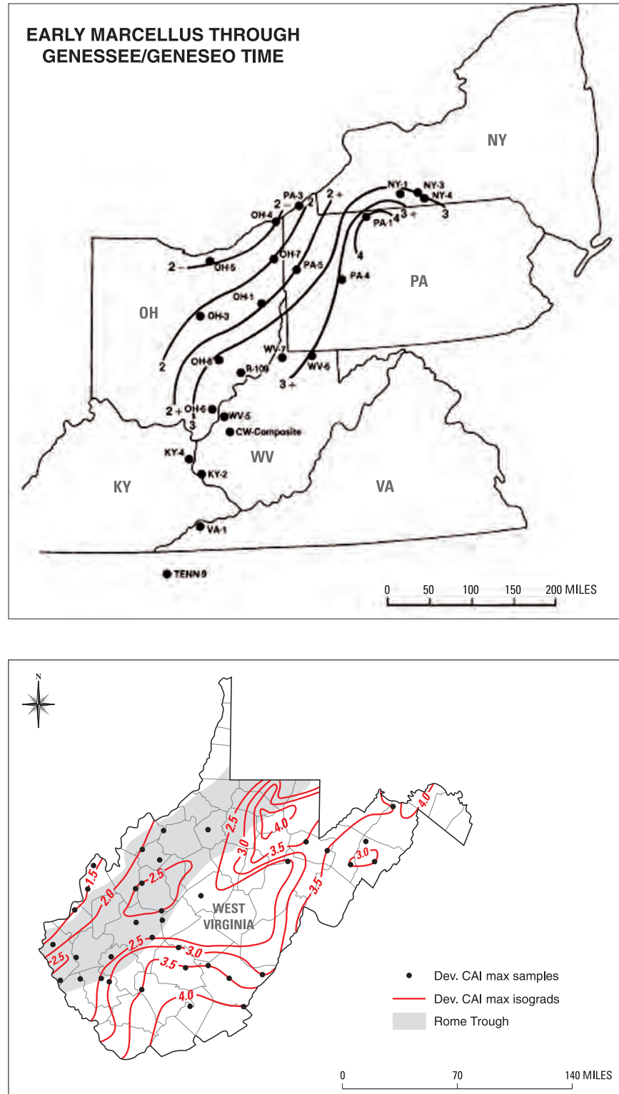
Figure 51. Top: values of Thermal Alteration Index (TAI) for the Marcellus-Genesee stratigraphic interval in the central Appalachian Basin; modified from Zielinski and McIver, 1982. Bottom: values of Conodont Alteration Index (CAI) for the Marcellus Shale in West Virginia; modified from Repetski and others, 2005.
