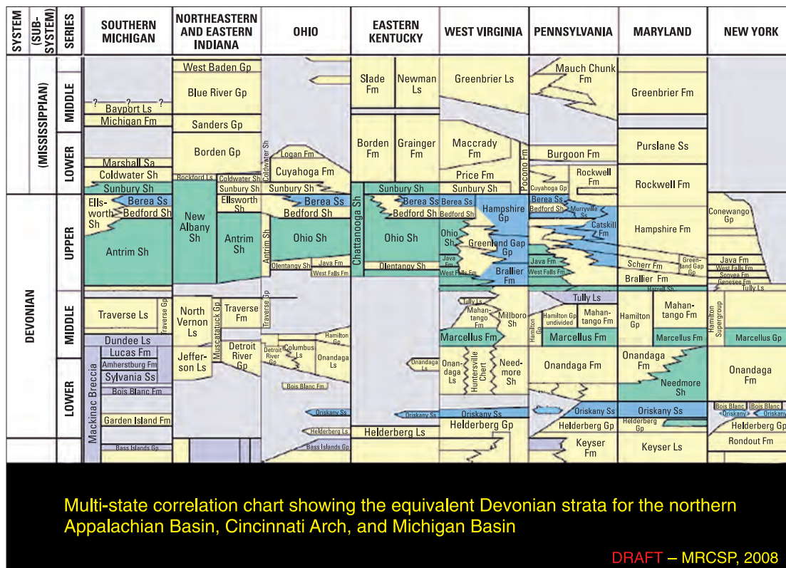
Figure 27. Multi-state correlation chart of Devonian strata in eastern U.S. The Middle-Upper Devonian Taghanic unconformity has removed much of the rock record in Ohio and adjoining states. Modified from Wickstrom and Carter, 2008.
