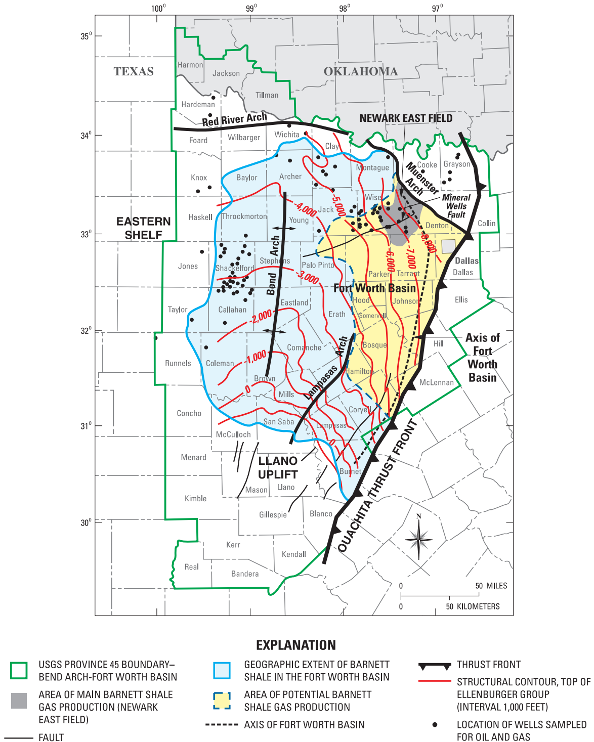
Figure 2. Fort Worth Basin showing the major geological features that influence the Barnett Shale and structural contours. The main producing area of the Newark East field is indicated by darker shading. Contours are drawn on top of the Ordovician Ellenburger Group; contour intervals equal 1,000 feet. Modified from Hill and others, 2007a, and Montgomery and others, 2005.
