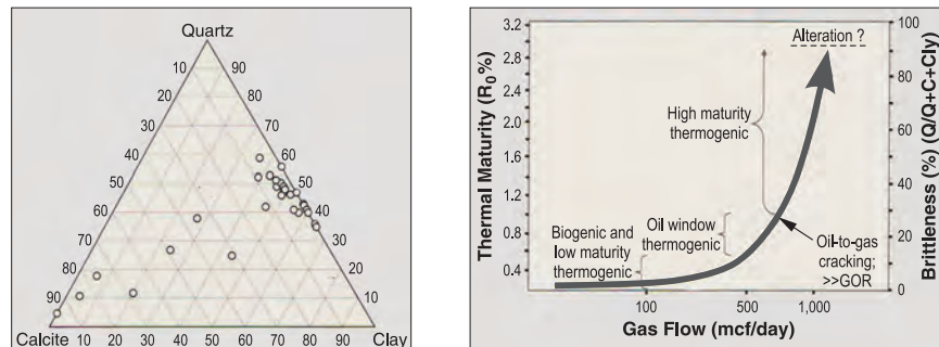
Figure 14a. Left: mineral content of the Barnett Shale in terms of quartz, clay minerals, and calcite. Right: relationship between gas flow and thermal maturity and shale brittleness ( Q/(Q+C+Cl) ). Modified from Jarvie and others, 2007.
