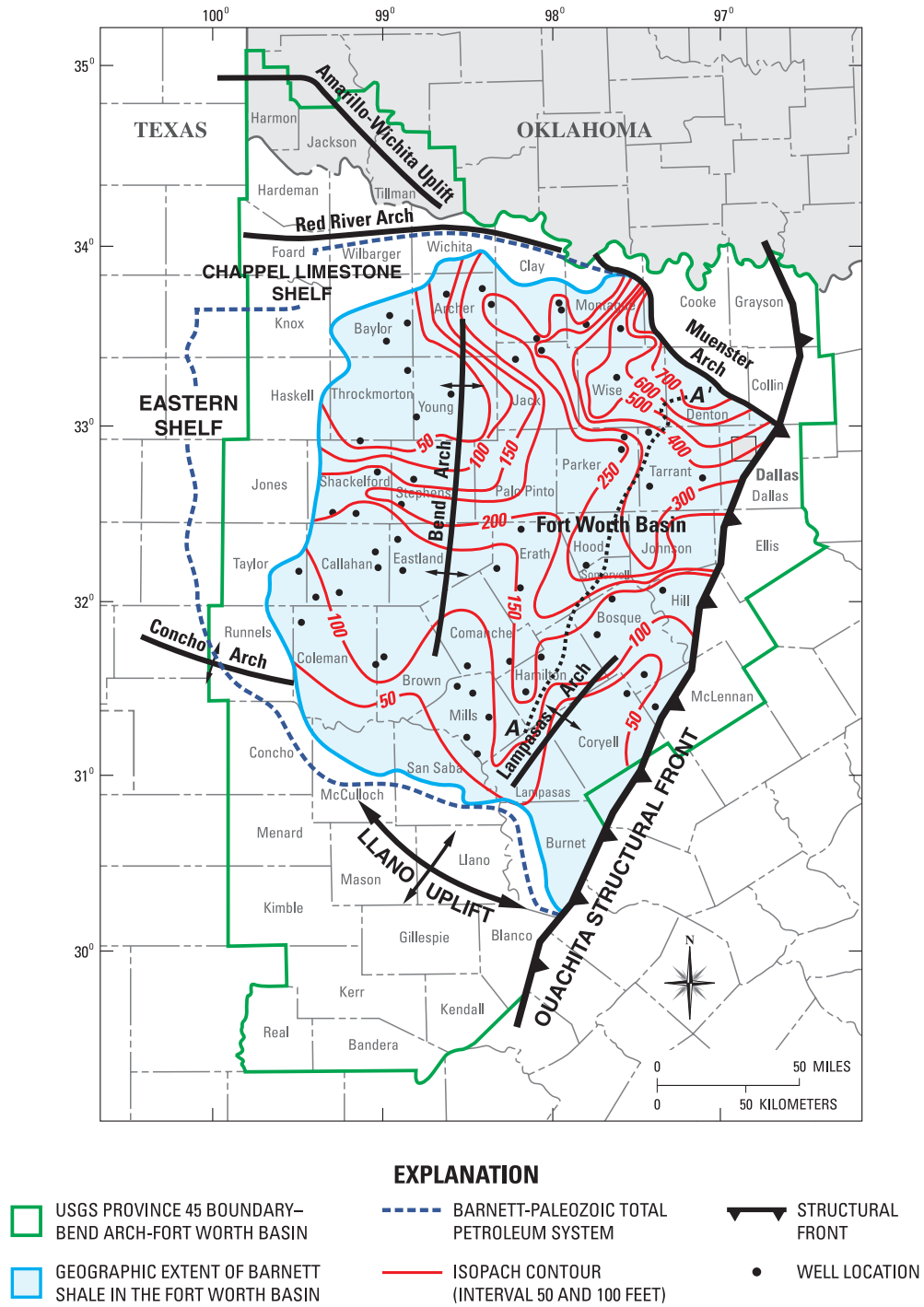
Figure 10. Thickness of Barnett Shale, isopach lines in red, contour interval equals 50 and 100 ft. Line A-A' marks the approximate axis of deposition. Modified from Barnett Shale Maps, 2007.
